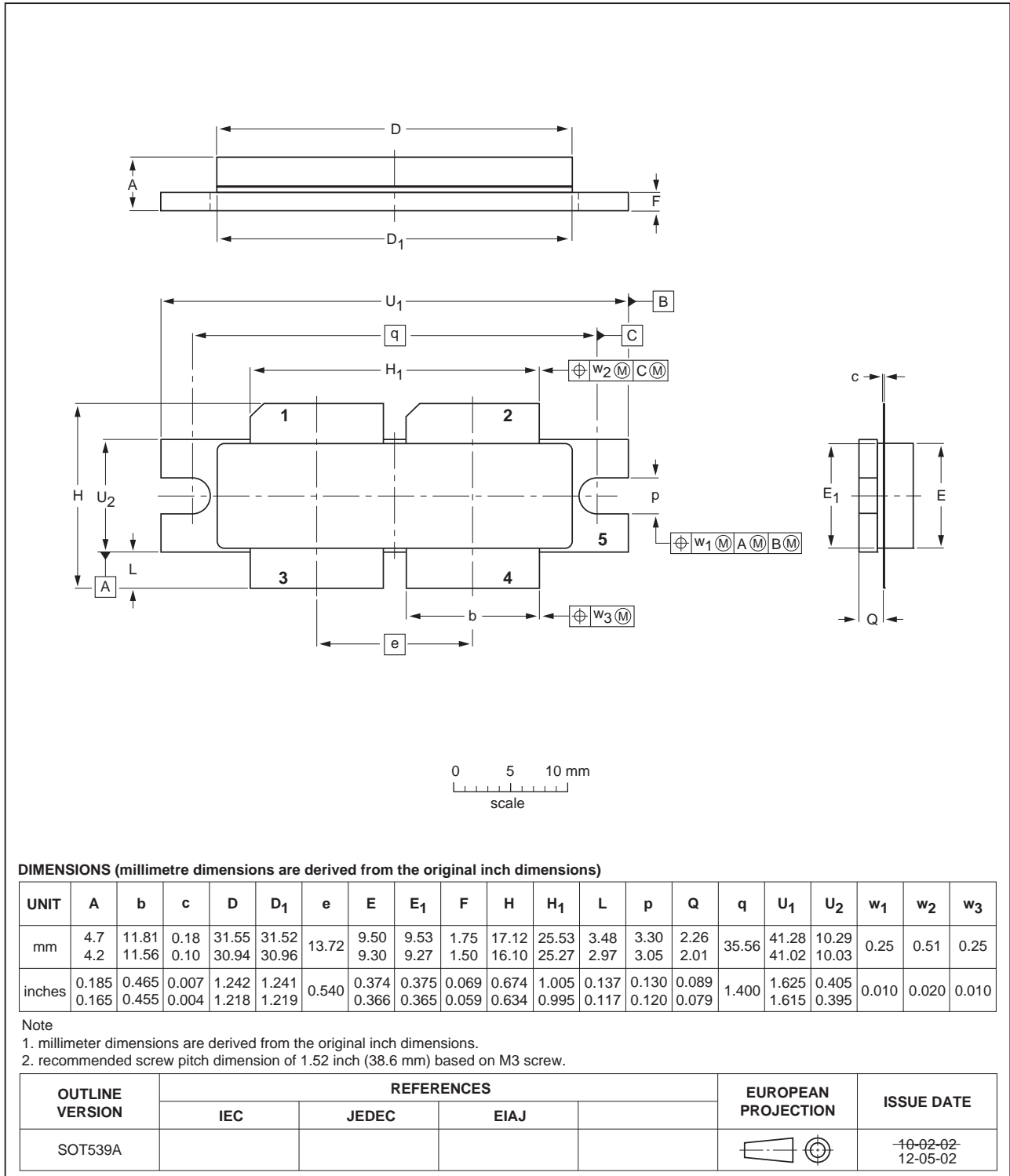
Fig 7. Package outline SOT539A
